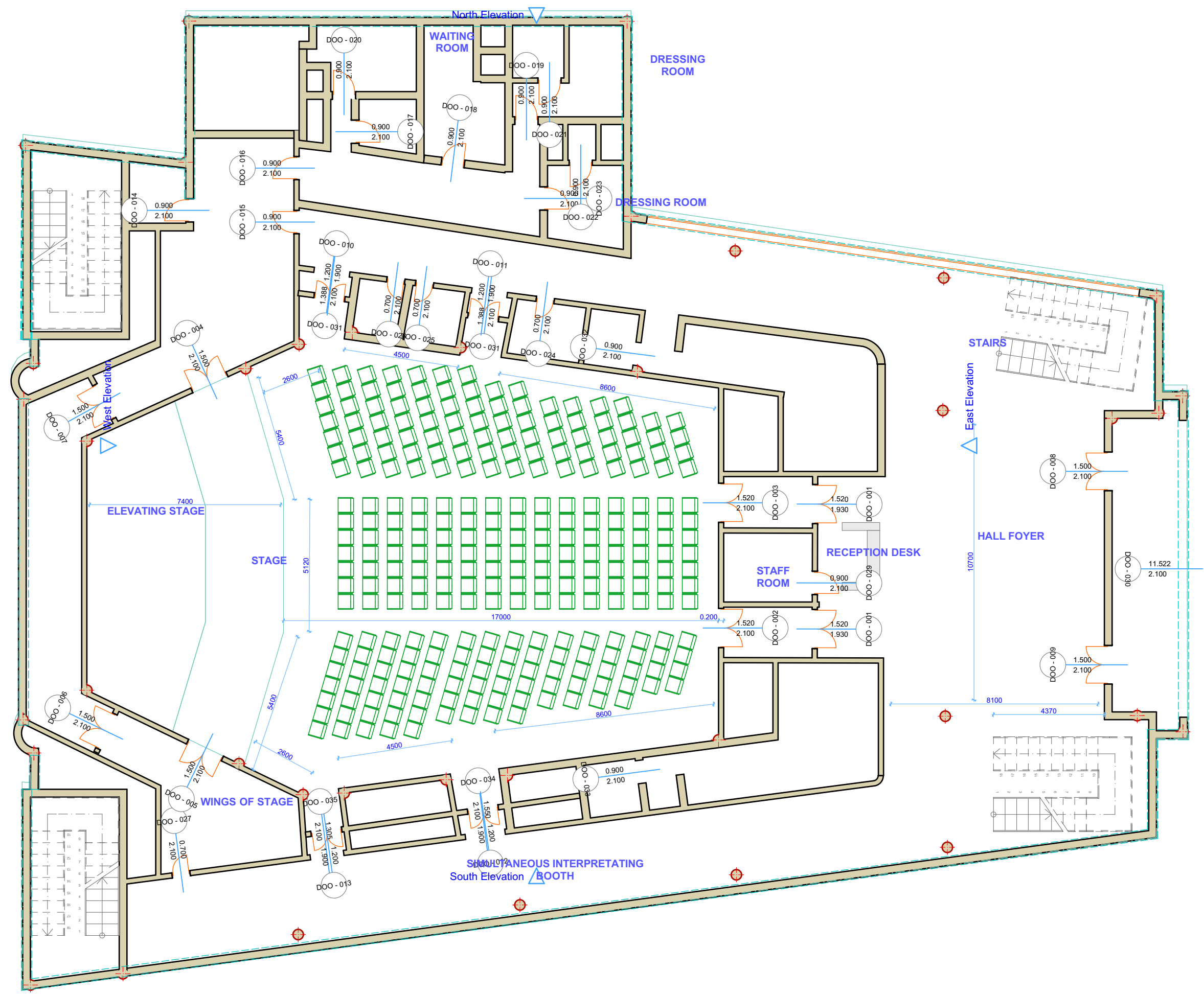
0. LEVEL 1 1:150
